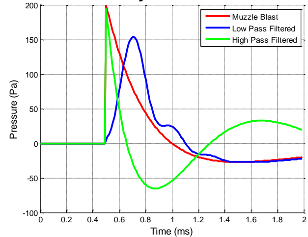
Electronically Filtered Muzzle Blast
