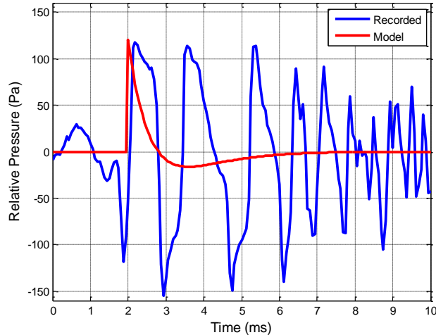
Recorded and Modeled Muzzle Blast
